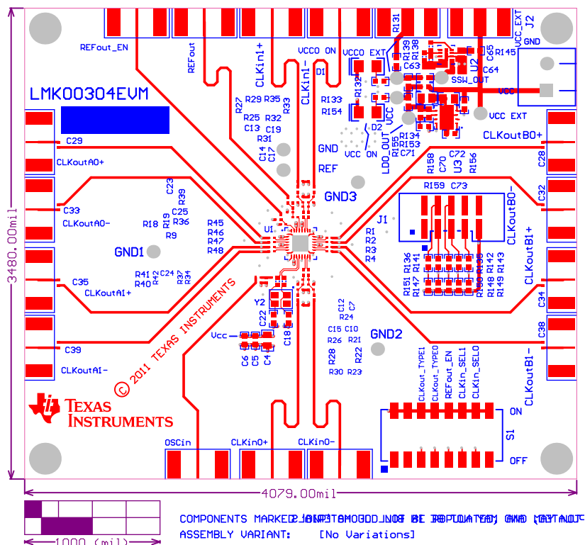
Figure 6: Top Side, Layer #1 (Not to scale)
