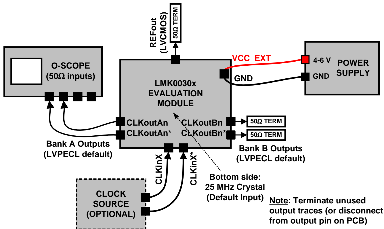
Figure 2: LMK00304 Evaluation Board Quick Start Setup
