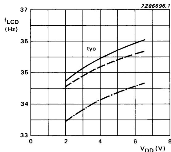
Fig. 19 Display frequency as a function of supply voltage; C_O = 1,5 nF (only PCF2112).
