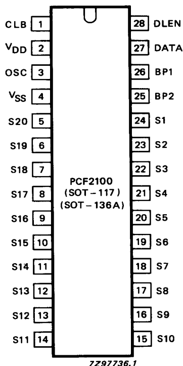
Fig. 2 Pinning diagram; PCF2100
