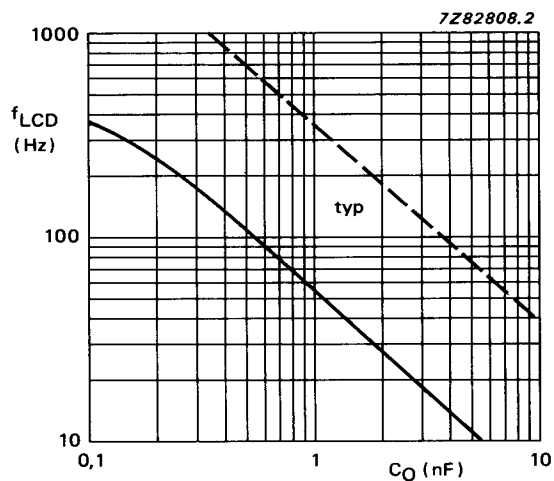
Fig. 20 Display frequency as a function of R_O and C_O ; T_{amb} = +25 °C; V_{DD} = 5 V.
