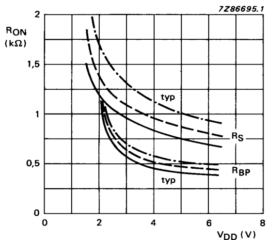
Fig. 22 Output resistance of backplane and segments.
