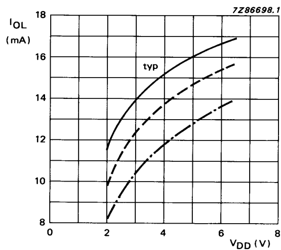
Fig. 23 Output current as a function of supply voltage (only PCF2112).
