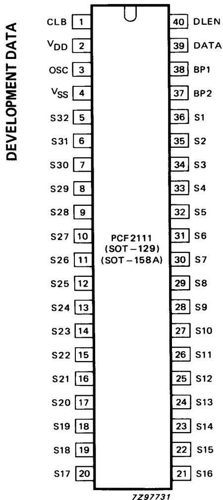
Fig. 7 Pinning diagram; PCF2111
