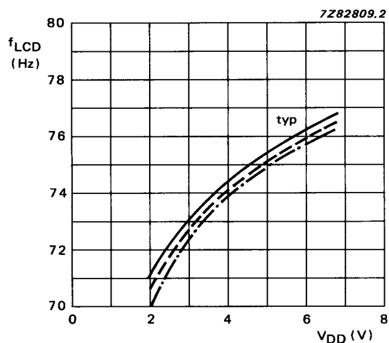
Fig. 18 Displays frequency as a function of supply voltage; C_O = 680 pF (except PCF2112).
