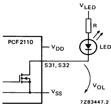
Fig. 11 LED driver circuitry.
