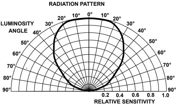
FIGURE 5. RADIATION PATTERN
