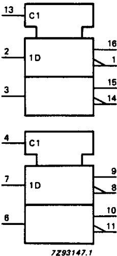
Fig.3 IEC logic symbol.
