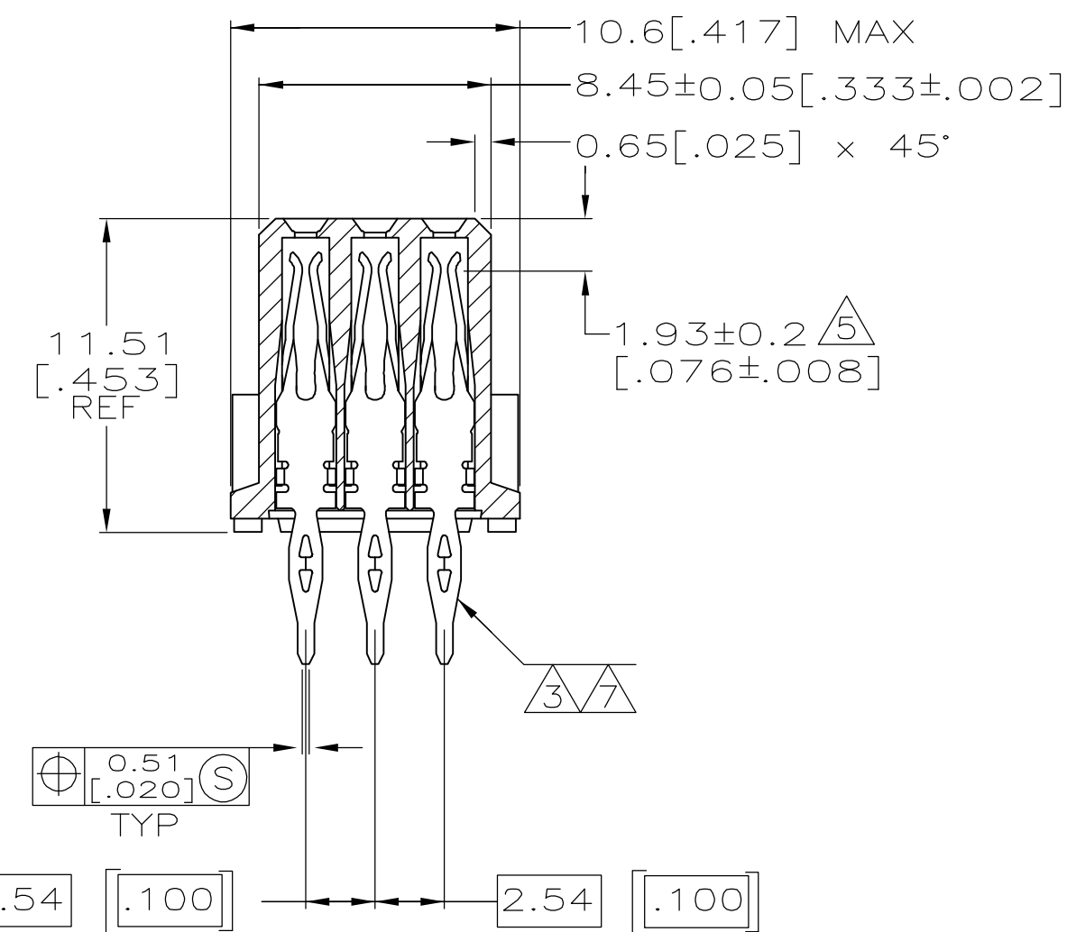
SECTION X-X
