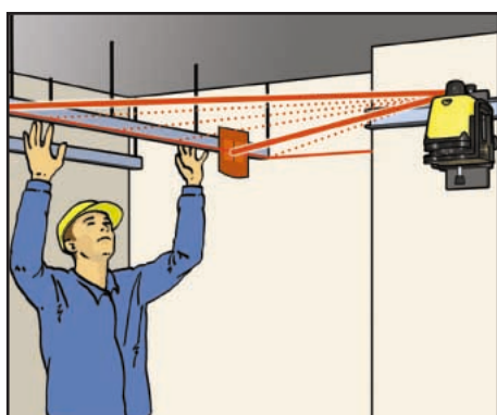
Interior leveling with use of wallmount.
