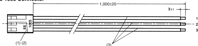
EE-1005 Connector
