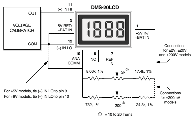
Figure 9. External Gain Adjustment
