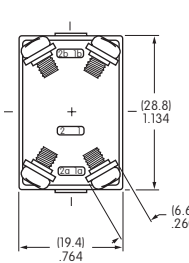
Double Pole
