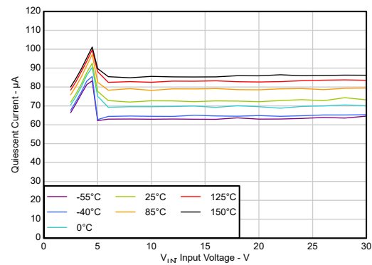
Figure 5-14. Quiescent Current vs Input Voltage (New Chip)
