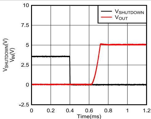
Figure 7-13. Enable Transient Response vs Time (New Chip)
