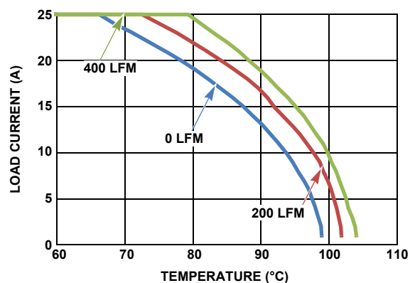
FIGURE 22. 12V_{IN} TO 2.5V_{OUT}
