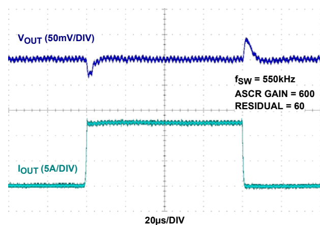
FIGURE 13. 1.8V TRANSIENT RESPONSE
