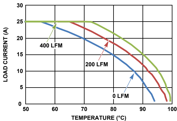
FIGURE 25. 12V_{IN} TO 5V_{OUT} , 727kHz
