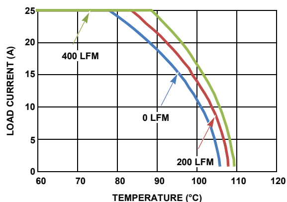
FIGURE 16. 12V_{IN} TO 1V_{OUT}
