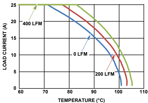
FIGURE 20. 12V_{IN} TO 1.8V_{OUT}
