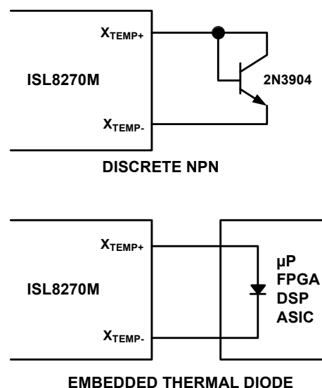
FIGURE 28. EXTERNAL TEMPERATURE MONITORING
