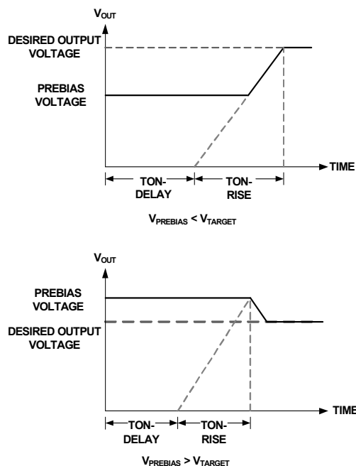
FIGURE 27. OUTPUT RESPONSES TO PREBIAS VOLTAGES
