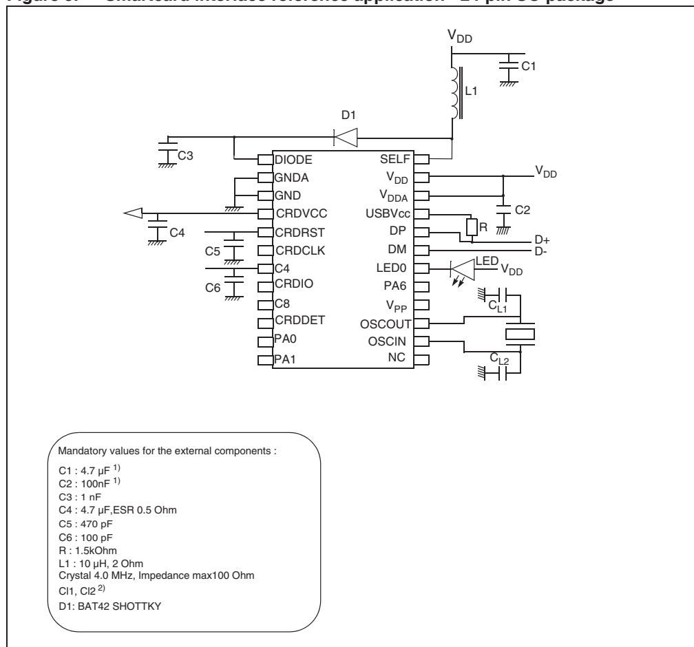
Figure 5. Smartcard interface reference application - 24-pin SO package
