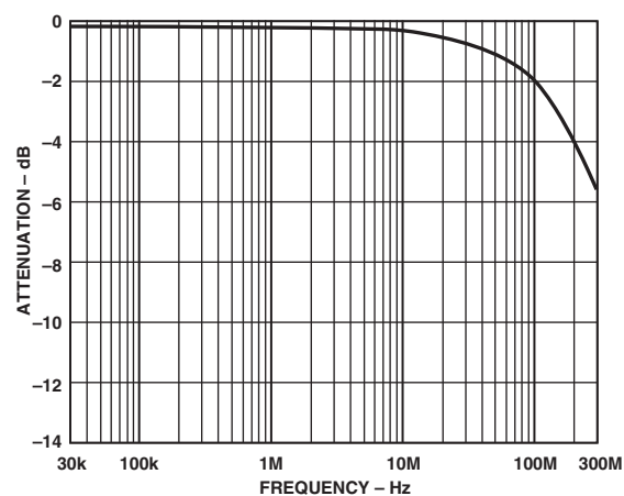
TPC 12. On Response vs. Frequency
