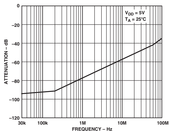
TPC 11. Off Isolation vs. Frequency
