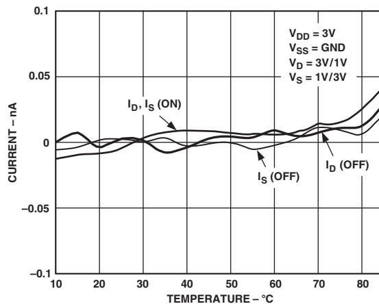
TPC 10. Leakage Currents as a Function of Temperature
