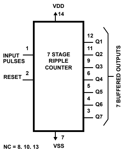
CD4024BMS
