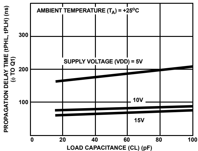
FIGURE 9. TYPICAL PROPAGATION DELAY TIME AS A FUNCTION OF LOAD CAPACITANCE ( \phi TO Q1))
