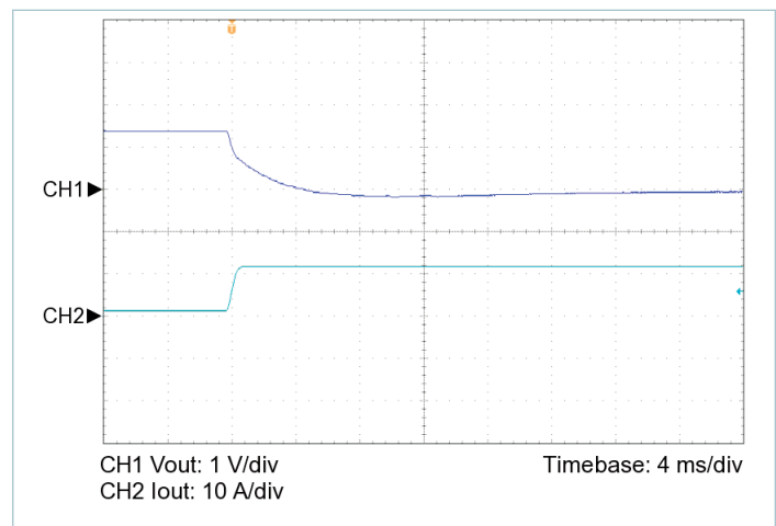
Figure 8 — 10% to 100% load transient response, V_{IN} = 48\text{ V} , nominal trim, C_{OUT\_EXT} = 250\text{ }\mu\text{F}
