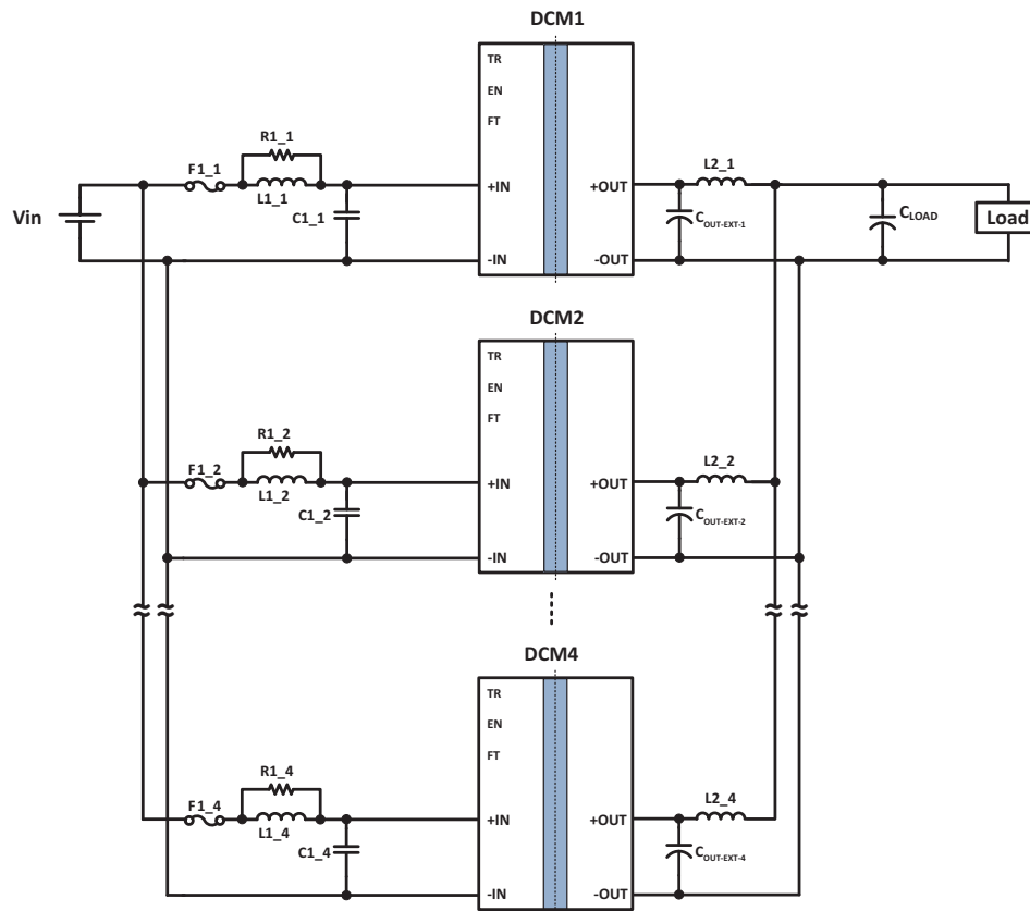
Typical Application 1: DCM3623x75H31C2yzz in an array of four units
