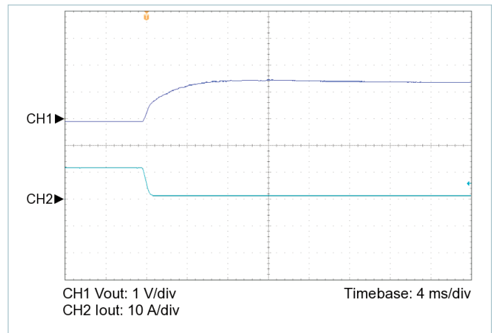
Figure 7 — 100% to 10% load transient response, V_{IN} = 48\text{ V} , nominal trim, C_{OUT\_EXT} = 250\text{ }\mu\text{F}
