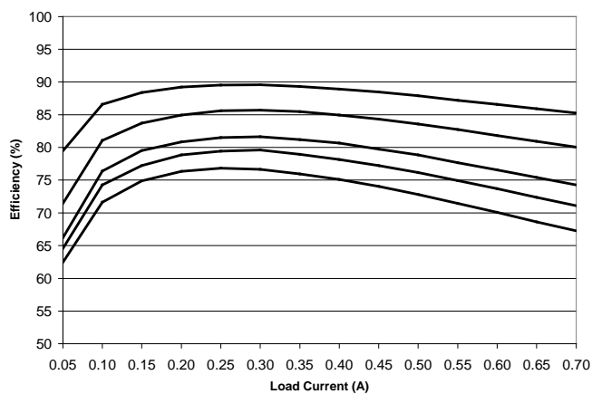
Efficiency Versus Load; V_{IN} = 5V , V_{OUT} (from top to bottom) 3.3V, 2.5V, 1.8V, 1.2V.
