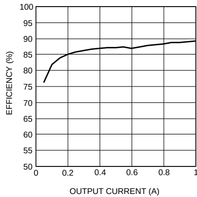
Figure 37. Efficiency V_{IN} = 24\text{ V} V_{OUT} = 5\text{ V}
