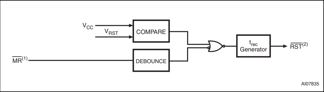
Figure 5. Block diagram
