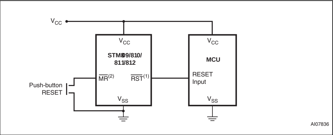
Figure 6. Hardware hookup
