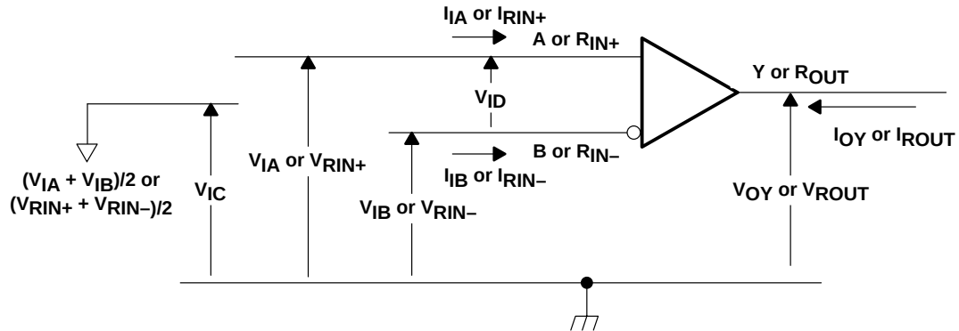
Figure 1. Voltage and Current Definitions
