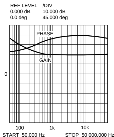
Figure 10. Error Amplifier Gain and Phase
