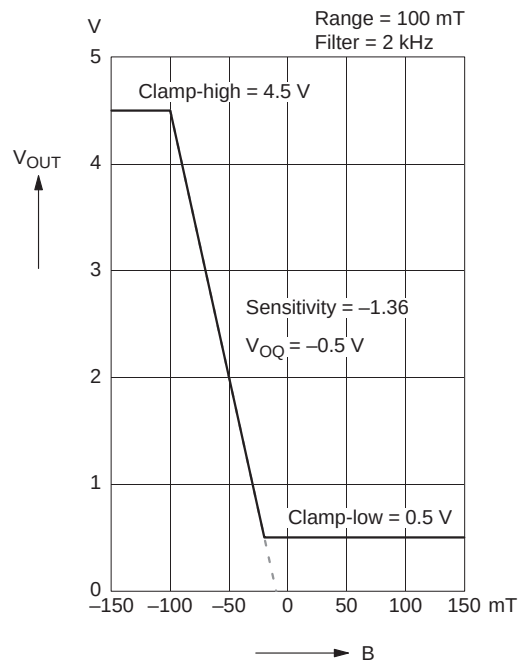
Fig. 2-5: Example for output characteristics
