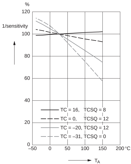
Fig. 3-7: Typical 1/sensitivity versus ambient temperature
