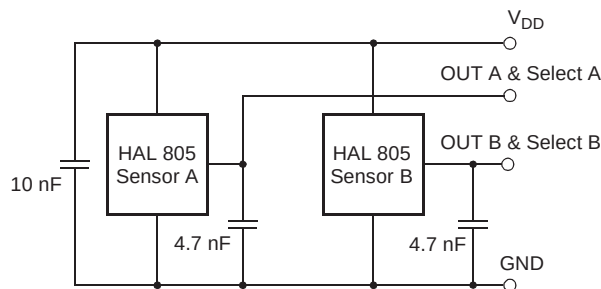
Fig. 4-2: Parallel operation of two HAL 805
