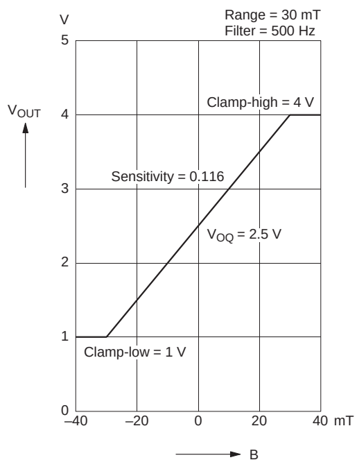
Fig. 2-4: Example for output characteristics
