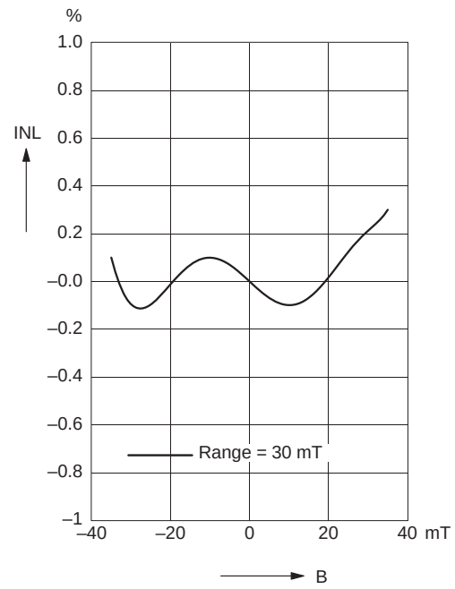
Fig. 3-9: Typical nonlinearity versus magnetic field
