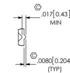
CRIMP DETAIL SCALE: 4:1 (TYP ALL CRIMPS)
