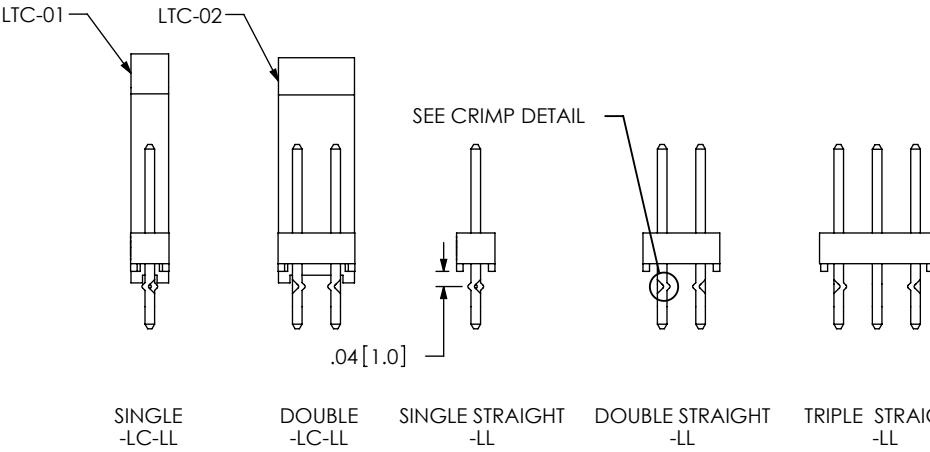
FIG 4 LOCKING LEAD (NOTE: END VIEWS SHOWN) (SAME AS FIG 1, DIFFERENT AS SHOWN)
