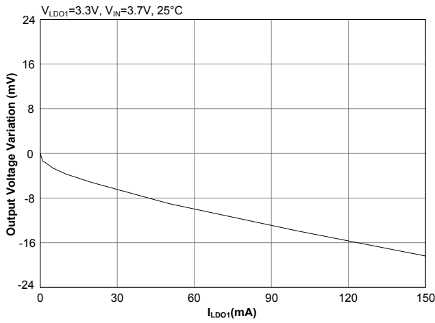
Load Regulation (LDO1)
