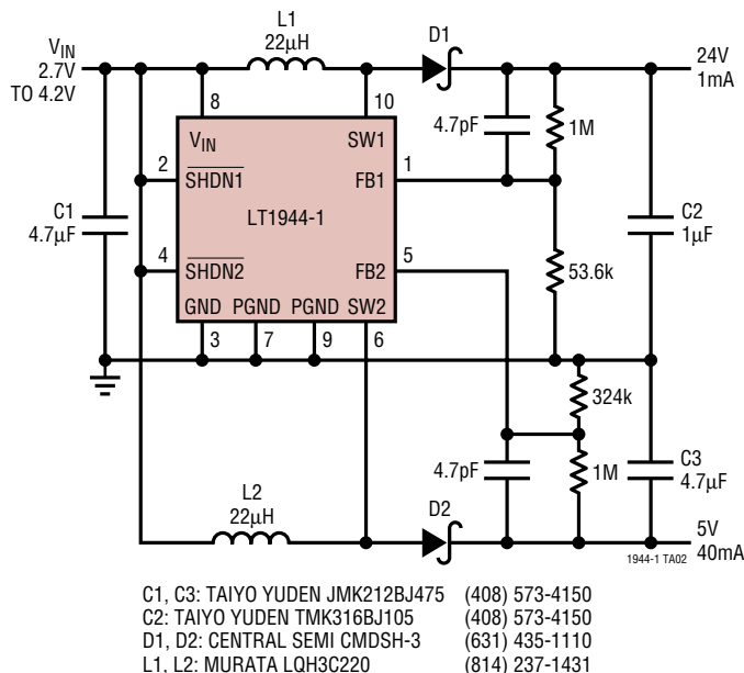
Dual Output (5V, 24V) Boost Converter
