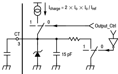
Figure 26. Oscillator
