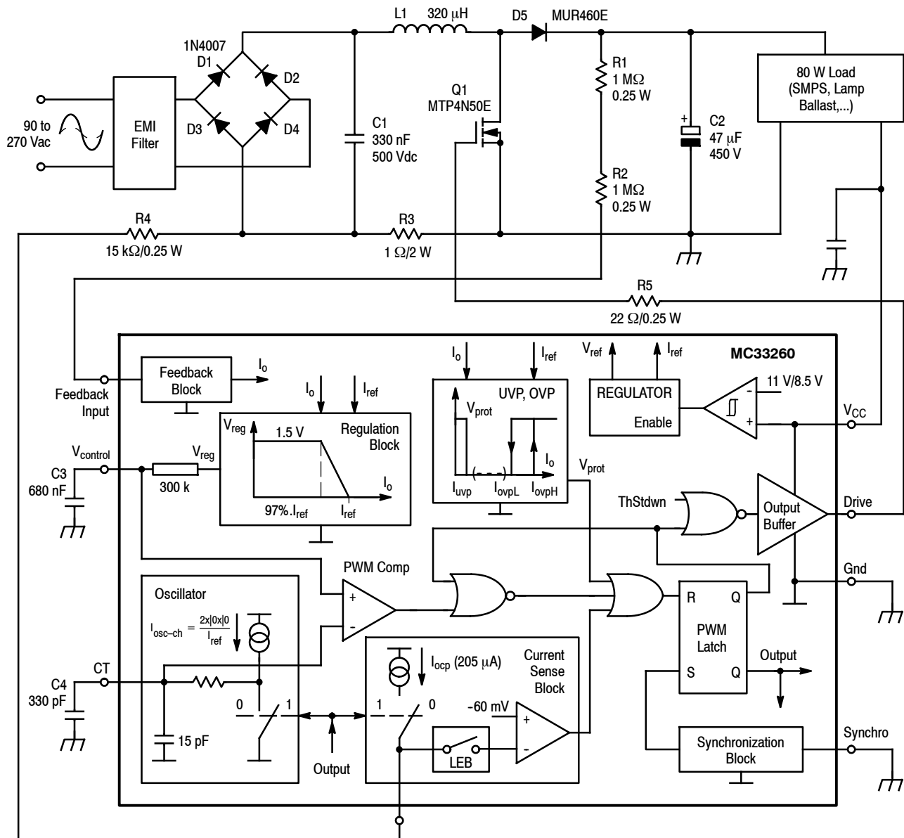
Figure 37. 80 W Wide Mains Power Factor Corrector
