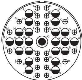
Insert Arrangement Service Rating Number of Contacts Contact Size 40-9 A 1 22 24 8 12 16
