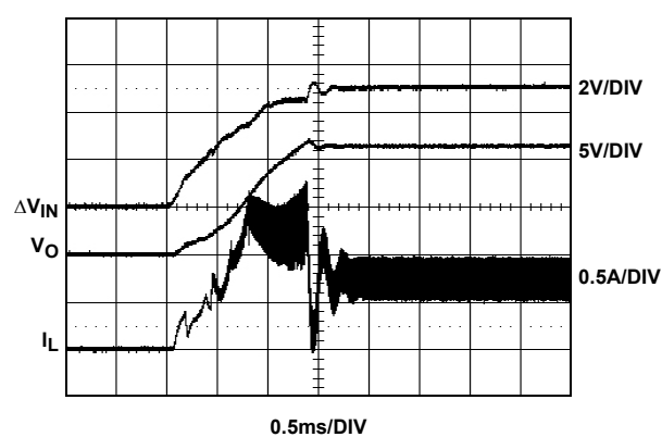
FIGURE 12. POWER-UP, V_{IN} = 5V , V_O = 12V , I_O = 300mA
