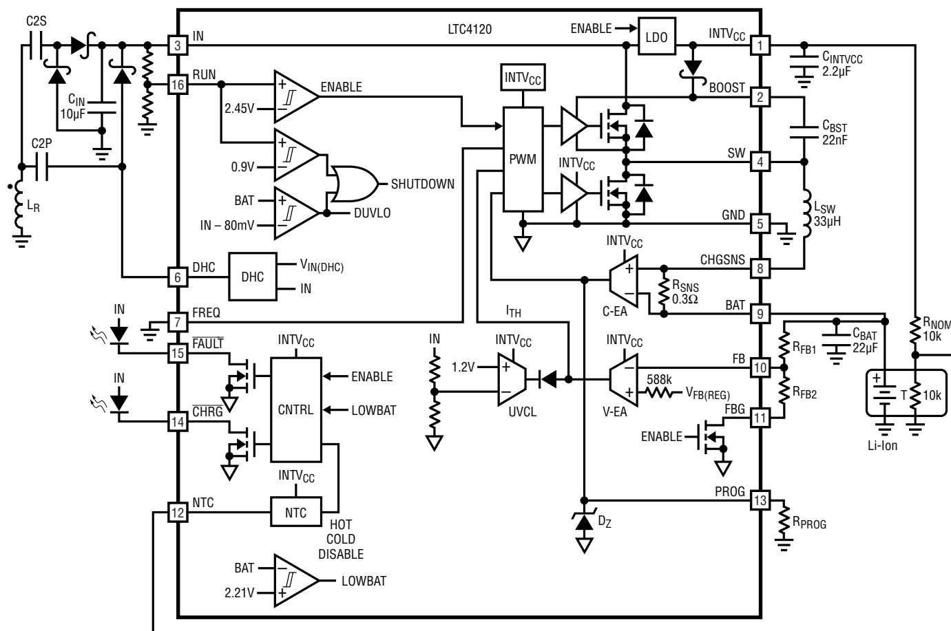
Figure 1. Block Diagram
