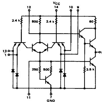
1/2 OF CIRCUIT SHOWN †
