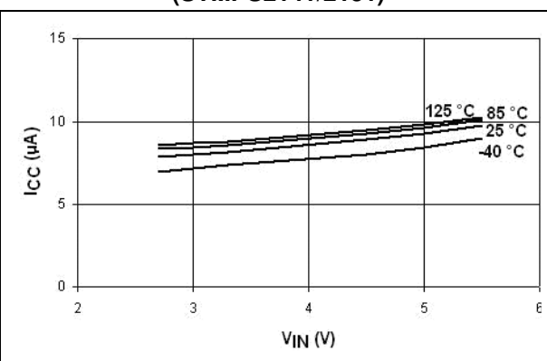
Figure 20. I_{CC} vs. temperature (disabled) (STMP2141/2151)
