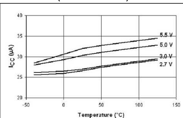
Figure 18. I_{CC} vs. temperature (enabled) (STMP2141/2151)
