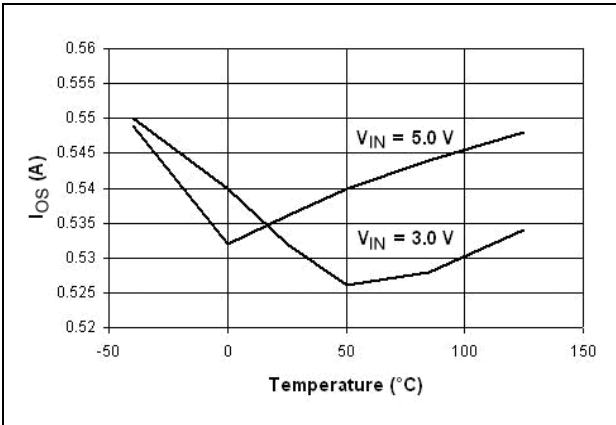
Figure 23. I_{OS} vs. temperature (STMP2141/2151)
