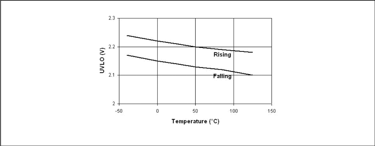
Figure 27. UVLO vs. temperature (STMPS2141/2151)
