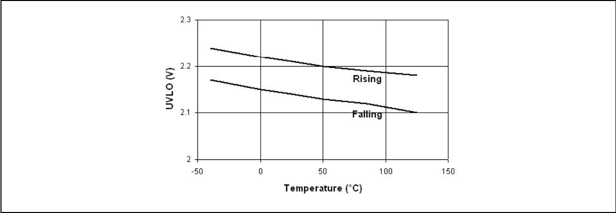
Figure 52. UVLO vs. temperature (STMPS2161/2171)
