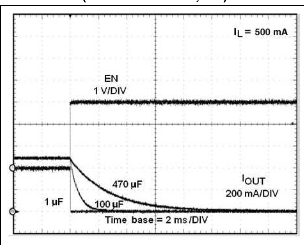
Figure 10. Current output turn-off delay time (STMP2141/2151, 3 V)
