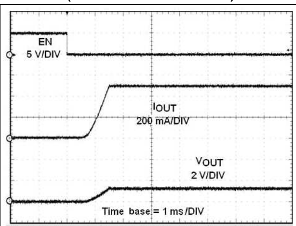
Figure 16. OC protection at V_{OUT} = 5.0\text{ V} (STMP2141/2151 - details)
