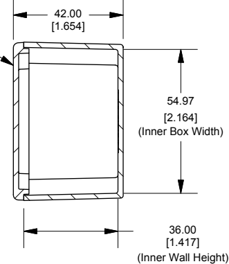
SECTION A-A End View of Assembly
