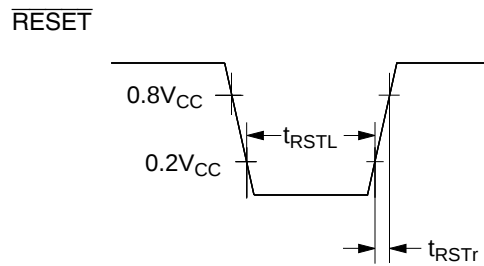
Figure 58 RESET Timing
