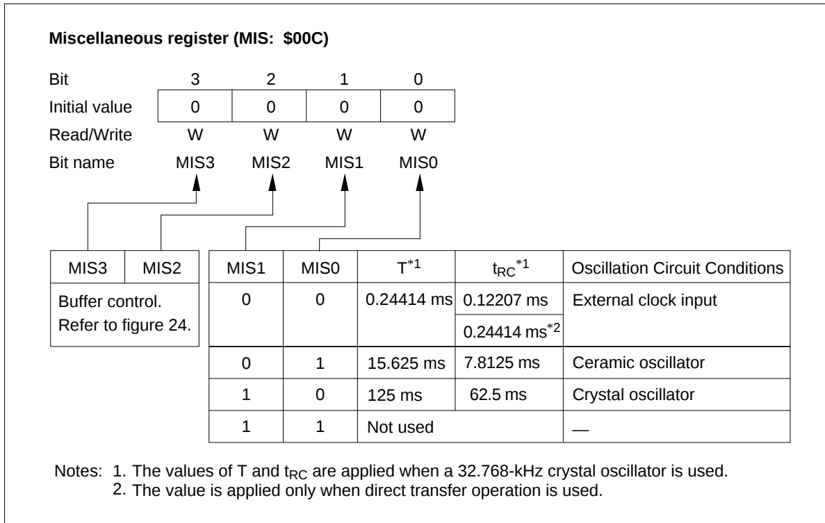
Figure 14 Miscellaneous Register
