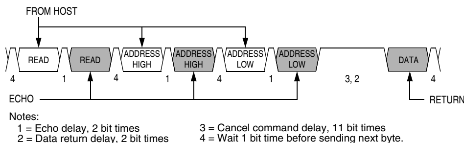
Figure 19-15. Read Transaction
