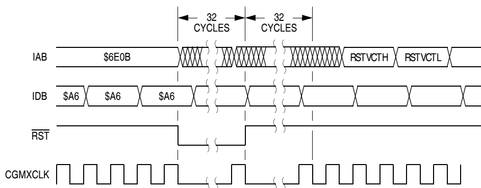
Figure 15-18. Wait Recovery from Internal Reset
