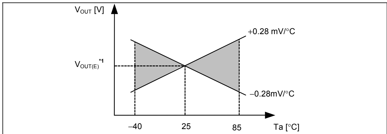
Figure 12 Typical example of the S-814A28A
