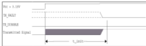
Power on initialization of GBIC, TX_DISABLE negated
