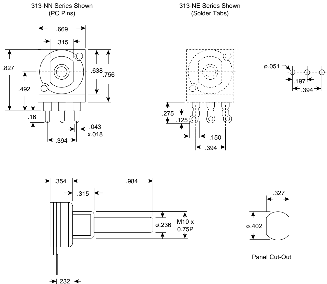
Dimensions (In.)
