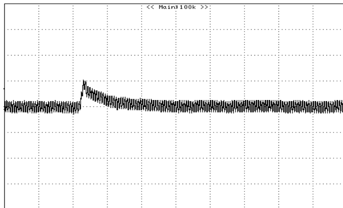
Figure 15: Typical transient response to step load change at 2.5A/μS from 100% to 50% of I_o , max at 12Vin, 5.0V out ( C_{out} = 1\mu\text{F ceramic} + 47\mu\text{F Ceramic} )(100mV/div, 50uS/div)
