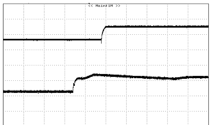
Figure 18: Turn on with Prebias 12Vin, 5V/0A out, V_{bias} = 3.3\text{Vdc} . (5mS/div)
