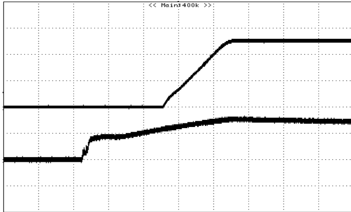
Figure 13: Turn on Using Input On/Off with external capacitors ( C_o=3000 \mu\text{F} ), 5.0V/3A out (resistive load)(2mS/div)
