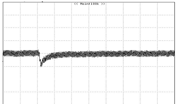
Figure 16: Typical transient response to step load change at 2.5A/μS from 50% to 100% of I_o , max at 12Vin, 5.0V out ( C_{out} = 1\mu\text{F ceramic} + 47\mu\text{F Ceramic} )(100mV/div, 50uS/div)
