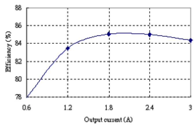
Figure 4: Converter efficiency vs. output current (12V in, 1.8V output voltage)
