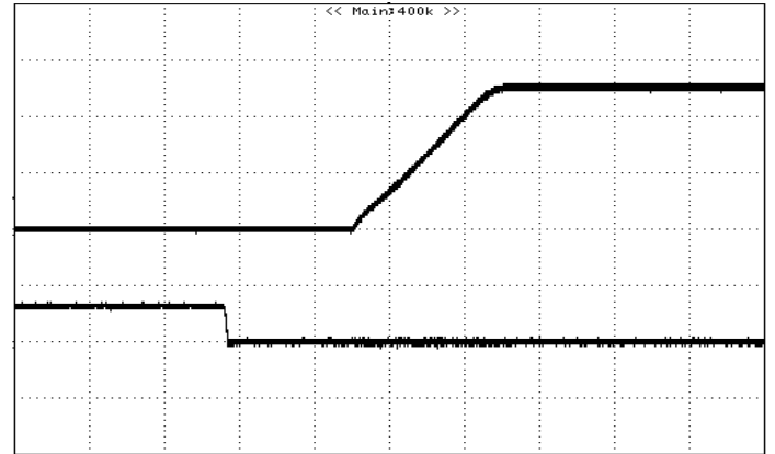
Figure 14: Turn on Using Remote On/Off with external capacitors ( C_o=3000 \mu\text{F} ), 5.0V/3A out(resistive load)(2mS/div)
