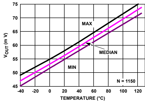
FIGURE 37. V_{OUT} LOW vs TEMPERATURE, V_+ = 5V , V_- = 0V , R_L = 1k
