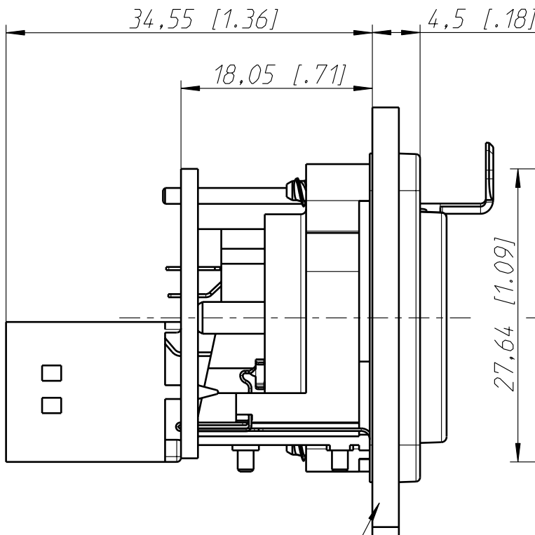
Frontplatte frontpanel
