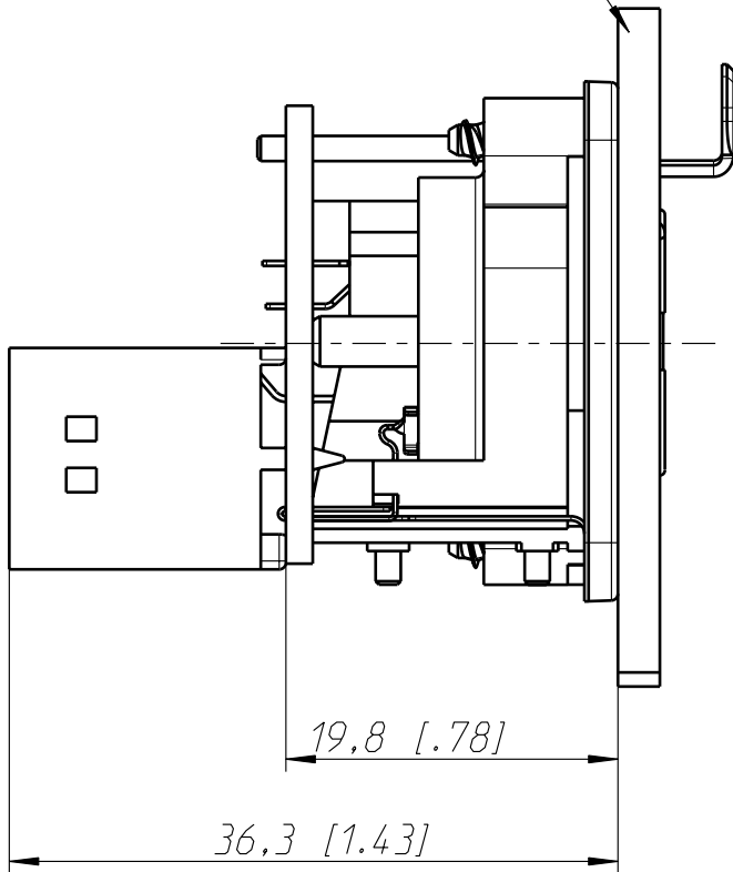
Frontplatte frontpanel
