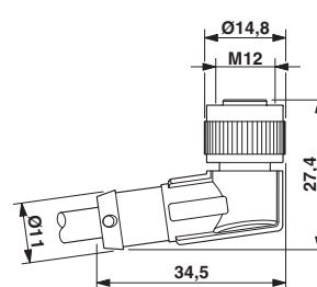
Dimensioned drawing
