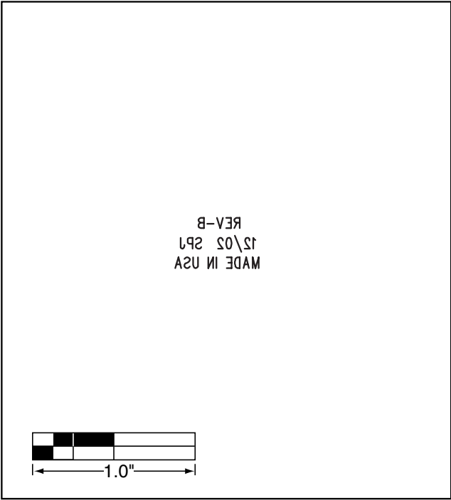
Figure 19. MAX2047 EV Kit Component Placement Guide—Bottom Silkscreen
