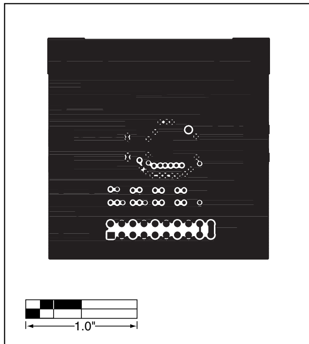
Figure 7. MAX2045 EV Kit PC Board Layout—Secondary Side
