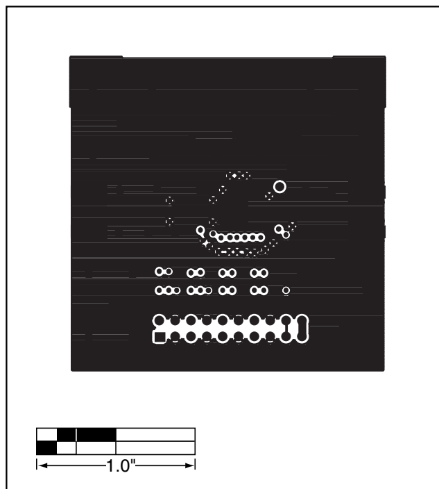
Figure 23. MAX2047 EV Kit PC Board Layout—Secondary Side
