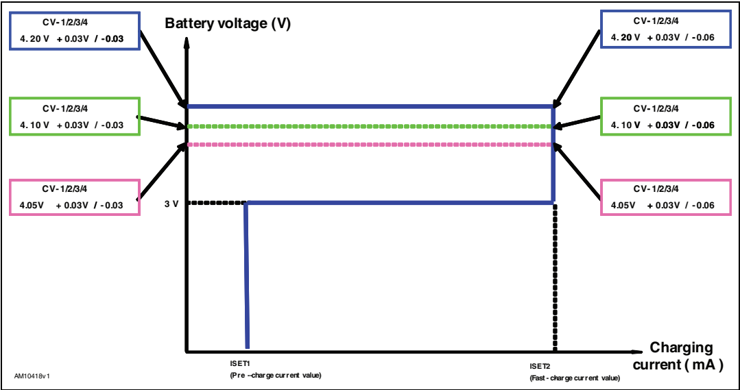
Figure 7. V-I characteristics
