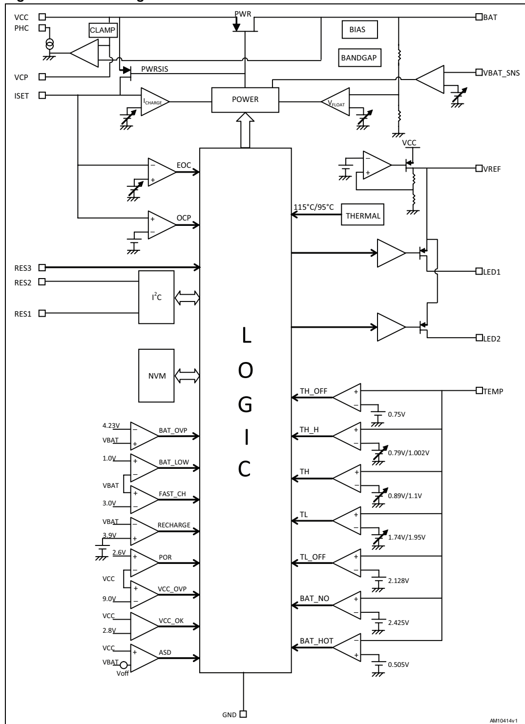
Figure 1. Block diagram
