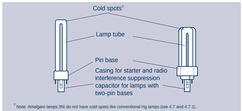
Technical design of OSRAM DULUX® S and OSRAM DULUX® T
