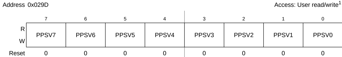
Figure 2-84. Port V Polarity Select Register (PPSV)
