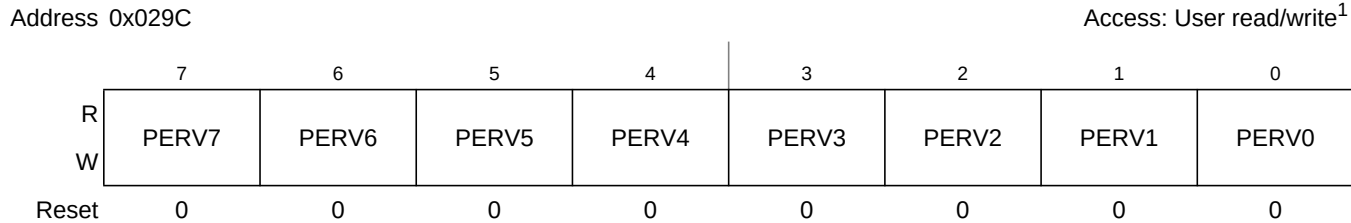
Figure 2-83. Port V Pull Device Enable Register (PERV)
