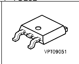
P-TO252
