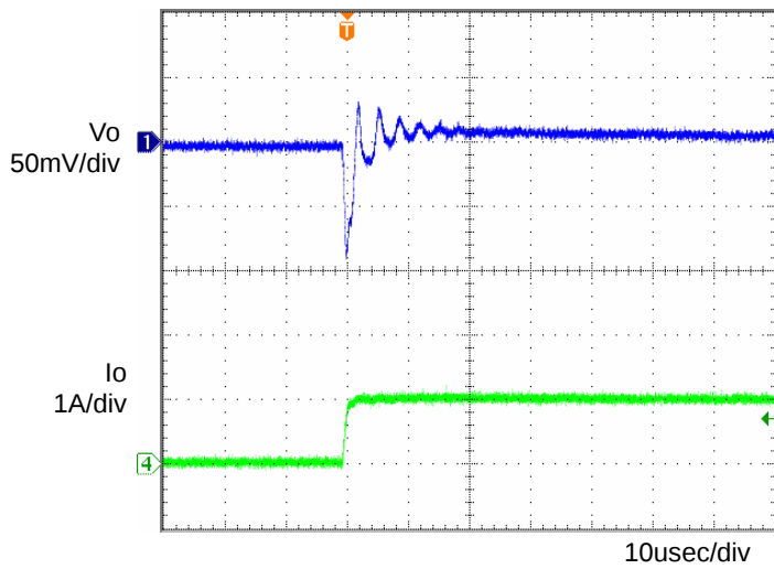
Fig.3 Transient Response (0→1.0A) C_o=1\mu\text{F} , T_a=-40^\circ\text{C}
