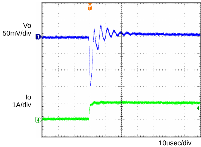
Fig.5 Transient Response (0→1.0A) C_o=1\mu\text{F} , T_a=105^\circ\text{C}
