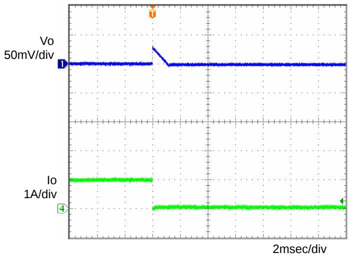
Fig.6 Transient Response (1.0→0A) C_o=1\mu\text{F} , T_a=-40^\circ\text{C}
