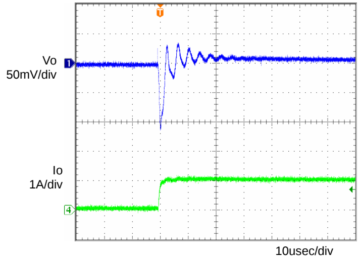
Fig.4 Transient Response (0→1.0A) C_o=1\mu\text{F} , T_a=25^\circ\text{C}
