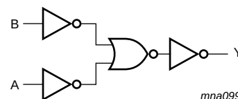
Fig 3. Logic diagram (one gate)
