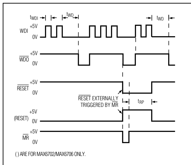
Figure 5. MAX6701/MAX6702/MAX6703/MAX6705/MAX6706/ MAX6707 Watchdog
