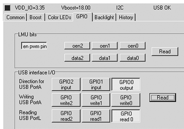
Figure 5. GPIO Tab
