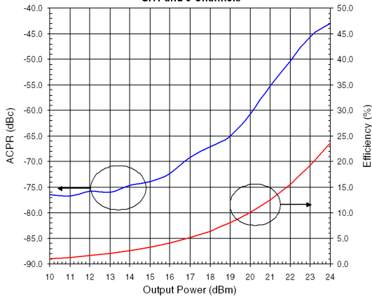
RF3807411 @ 882 MHz W-CDMA 64 Channels and No Clipping
